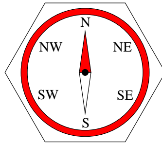
Figure 3: The COSMOS compass.
